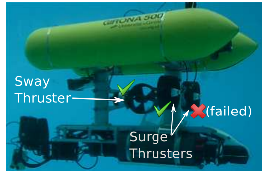
Fig. 1. The Girona500 AUV equipped with 5 thrusters (3 are visible in the photo). In our experiment, one of the surge thrusters is broken.
